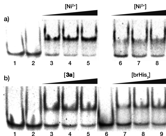
Figure 2. Comparative EMSA analysis of the DNA-binding processes. a) Lanes 1–8: AP1 hs -A/T (0.1 \mu M); lane 2–5: brHis 2 (1 \mu M) and 3a (1 \mu M); lanes 3–5: 0.6, 1, and 1.6 \mu M of Ni(ClO 4 ) 2 ; lanes 6–8: brHis 2 (1 \mu M), 3b (1 \mu M), and 0.6, 1, and 1.6 \mu M of Ni(ClO 4 ) 2 , respectively. b) Lanes 1–9: AP1 hs -A/T (0.1 \mu M); lane 2–5: brHis 2 (0.8 \mu M) and Ni(ClO 4 ) 2 (1.6 \mu M); lanes 3–5: 0.8, 1, and 1.6 \mu M of 3a ; lanes 6–9: 3a (0.8 \mu M) and Ni(ClO 4 ) 2 (1.6 \mu M); lanes 7–9: 0.8, 1, and 1.6 \mu M of brHis 2 . The procedure for fluorescence EMSA experiments involved the addition of peptide solutions in Tris-HCl (20 mM, pH 7.5) to a solution of Tris-HCl (18 mM, pH 7.5) containing KCl (90 mM), MgCl 2 (1.8 mM), glycerol (9%), BSA (0.11 mg mL -1 ), NP-40 (2.25%), and DNA (100 nM; 4 ^{\circ} C, 30 min) and loading into the gel. Products were resolved by PAGE analysis on a 10% non-denaturing polyacrylamide gel and 0.5X tris/borate/EDTA (TBE) buffer over 40 minutes at 4 ^{\circ} C and by staining with SybrGold (5 \mu L in 50 mL of TBE) for 10 minutes, followed by fluorescence visualization. Note that we needed to run the EMSA experiments in the absence of EDTA to avoid sequestration of the nickel cation; this is the reason for the smearing of the bands. Sequence of AP1 hs -A/T: 5'-ACGAACG TCA T-AATT CT CT-3' (peptide binding site in italics and minor-groove binding site underlined, only one strand shown).
